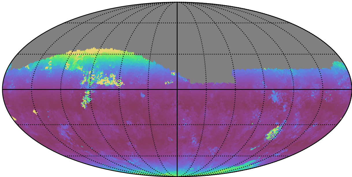
too_ignore_100_4v3.4_10yrs Yr 1 z band: Median airmass
