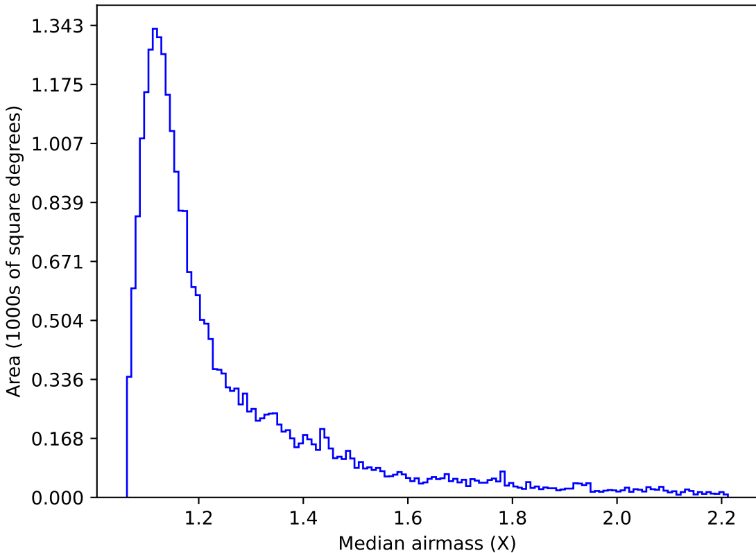
too_ignore_100_4v3.4_10yrs Yr 1 z band: Median airmass
