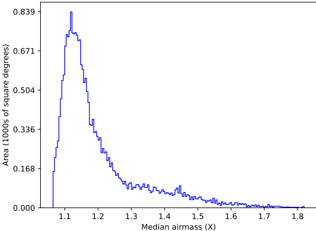
too_ignore_100_4v3.4_10yrs Yr 1 y band: Median airmass
