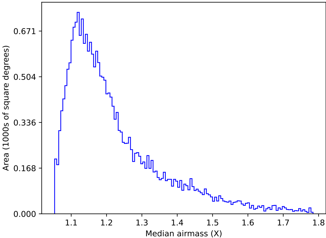
too_ignore_100_4v3.4_10yrs Yr 1 u band: Median airmass
