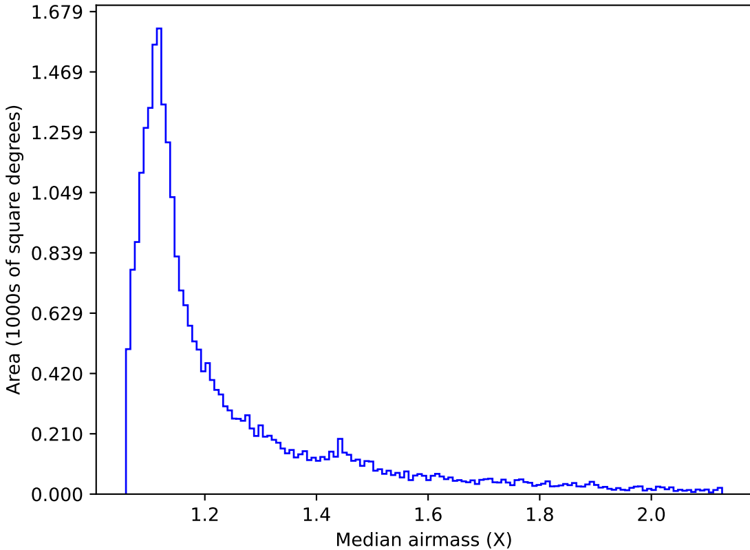
too_ignore_100_4v3.4_10yrs Yr 1 r band: Median airmass
