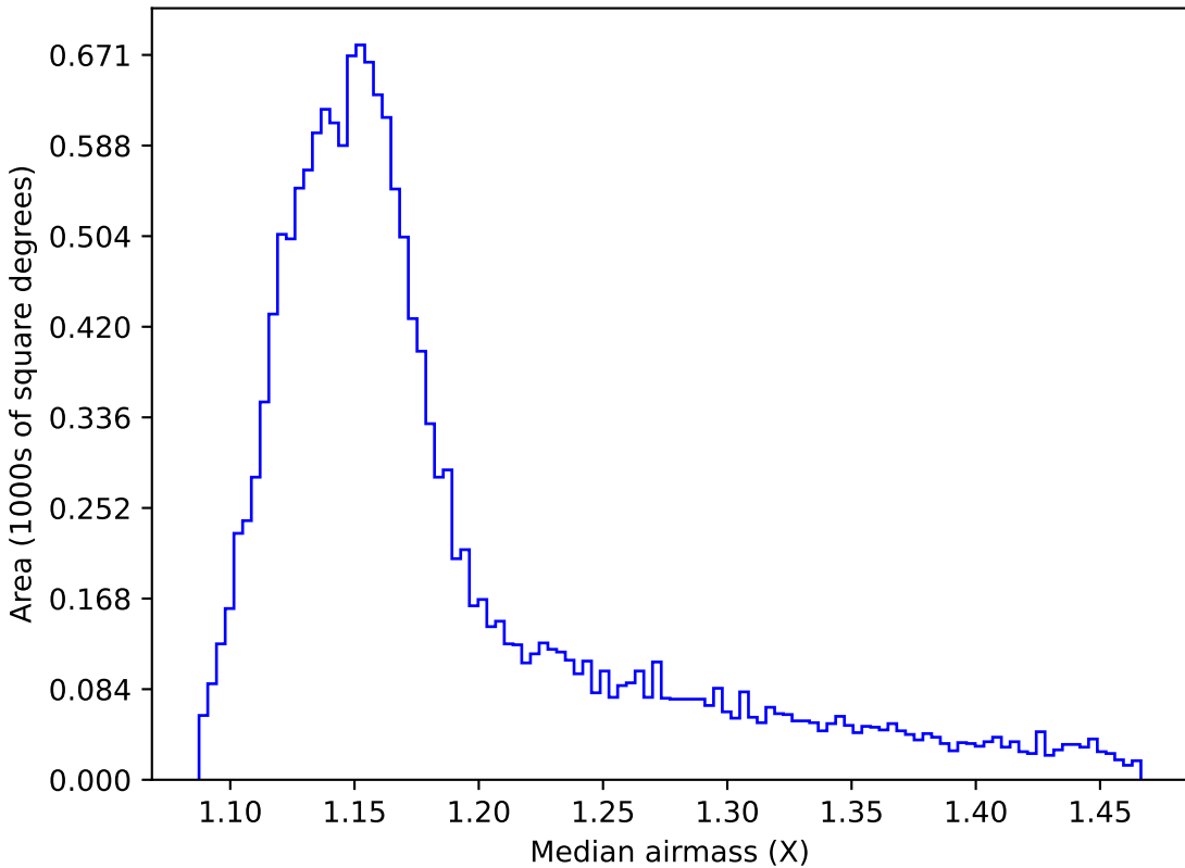
too_ignore_100_4v3.4_10yrs WFD z band: Median airmass
