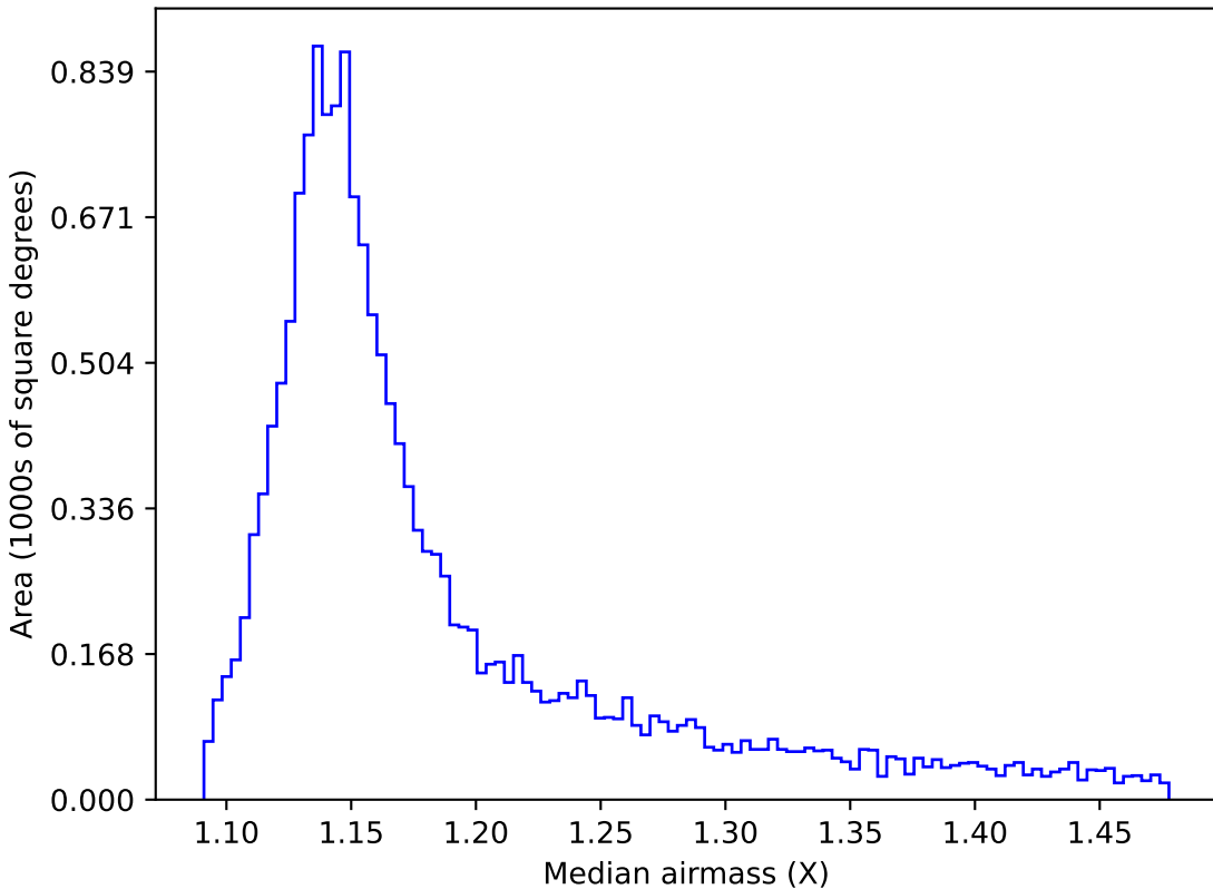
too_ignore_100_4v3.4_10yrs WFD y band: Median airmass
