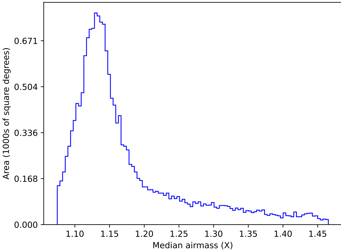
too_ignore_100_4v3.4_10yrs WFD r band: Median airmass
