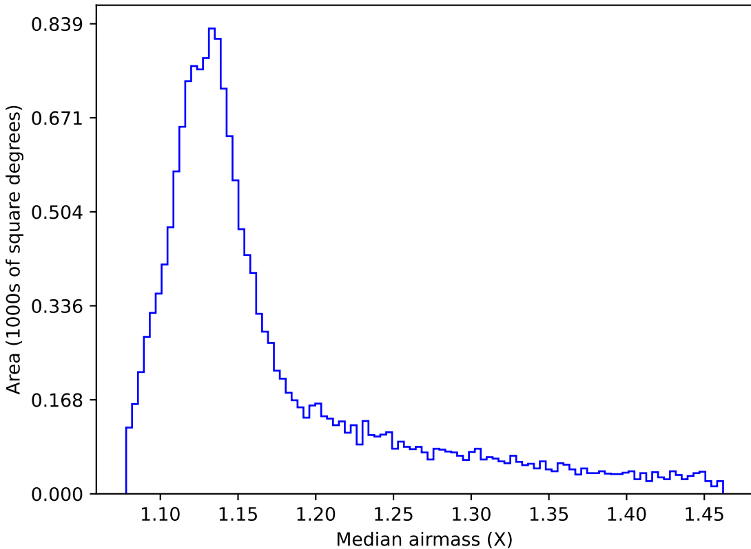
too_ignore_100_4v3.4_10yrs WFD i band: Median airmass
