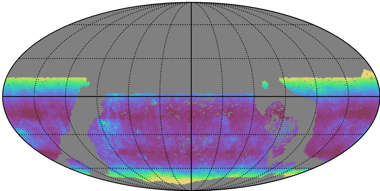
too_ignore_100_4v3.4_10yrs WFD g band: Median airmass
