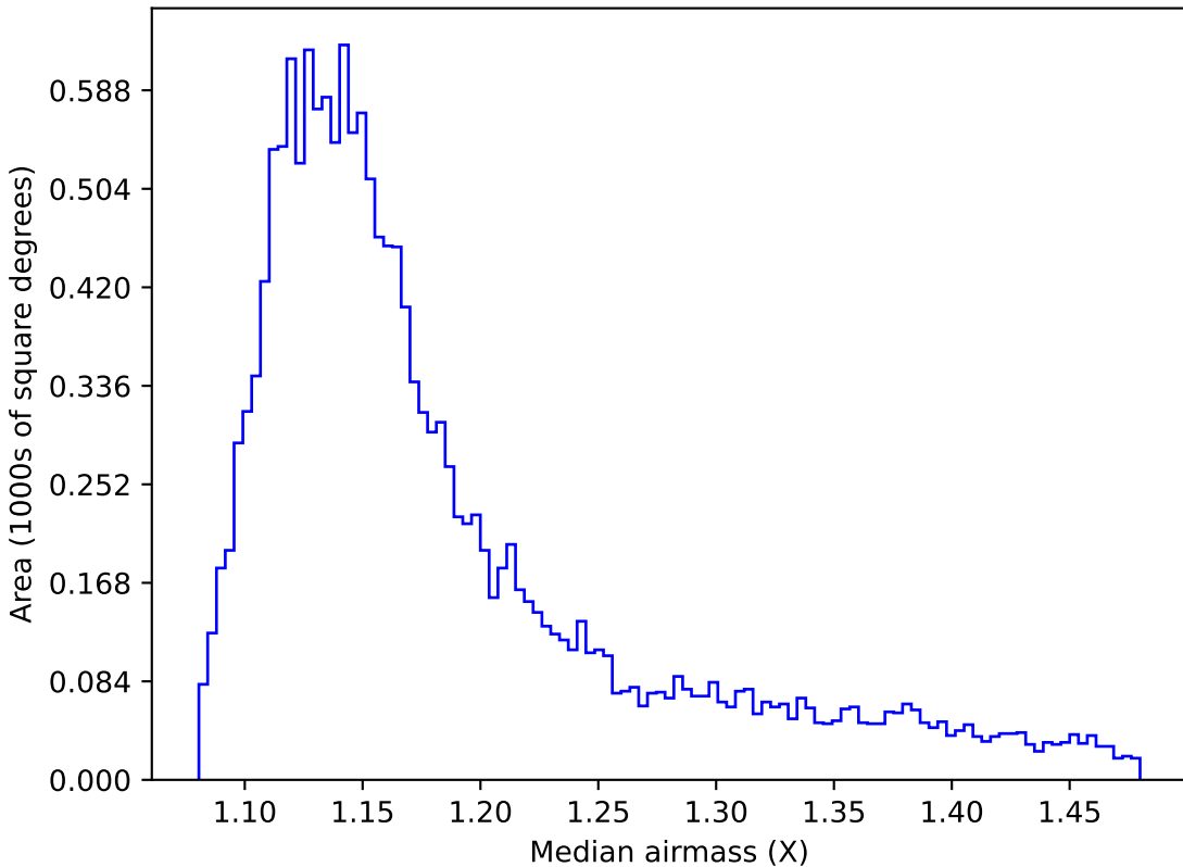
too_ignore_100_4v3.4_10yrs WFD g band: Median airmass
