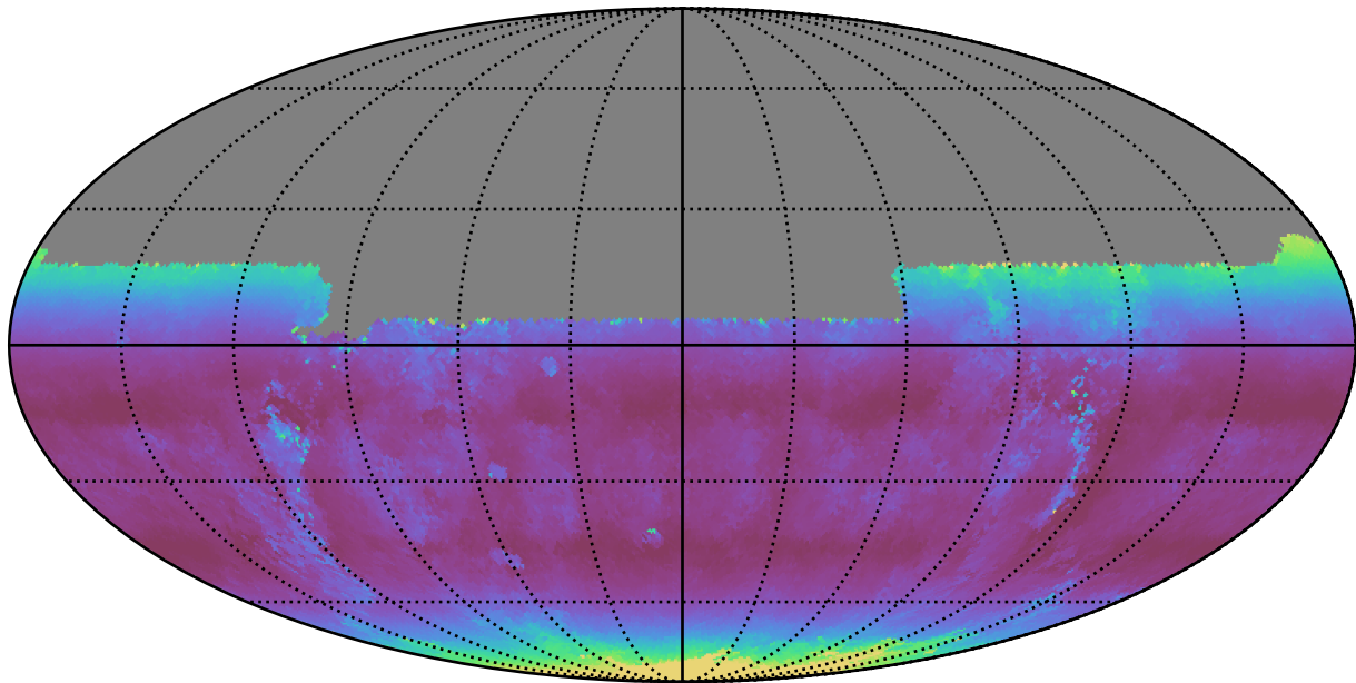
too_ignore_100_4v3.4_10yrs All sky u band: Median airmass
