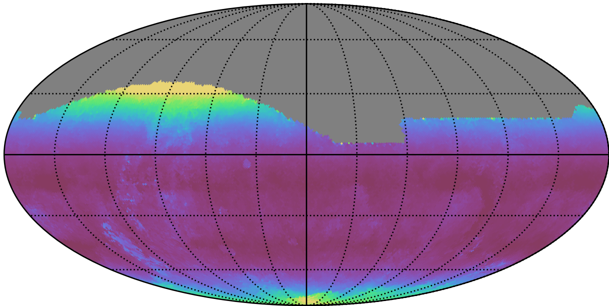
too_ignore_100_4v3.4_10yrs All sky g band: Median airmass
