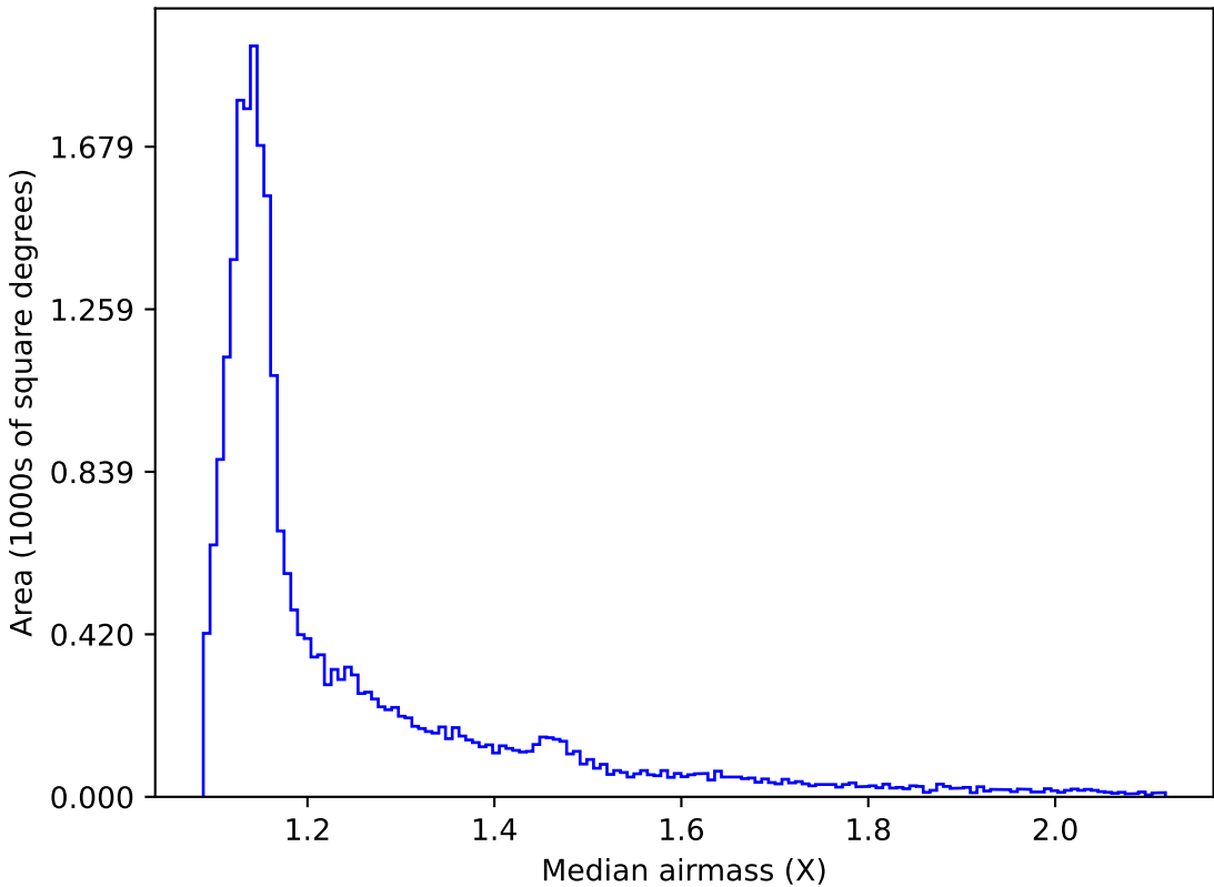
too_ignore_100_4v3.4_10yrs All sky all bands: Median airmass
