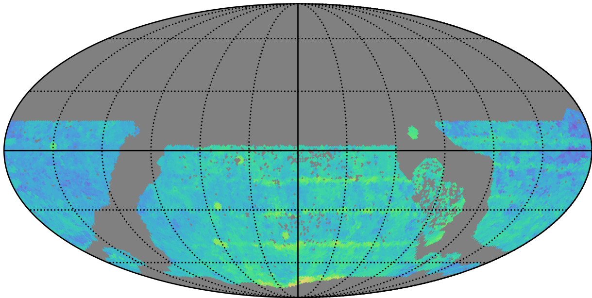
too_ignore_100_4v3.4_10yrs WFD z band: Median Season Length
