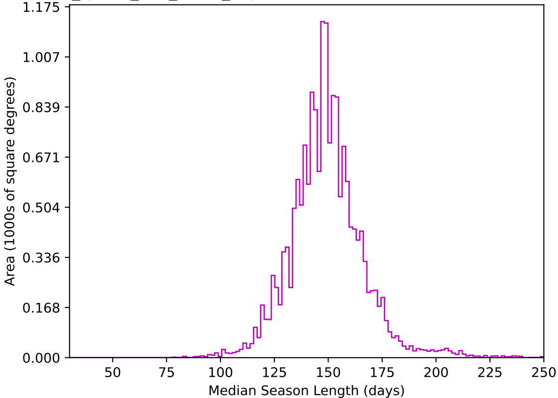
too_ignore_100_4v3.4_10yrs WFD z band: Median Season Length
