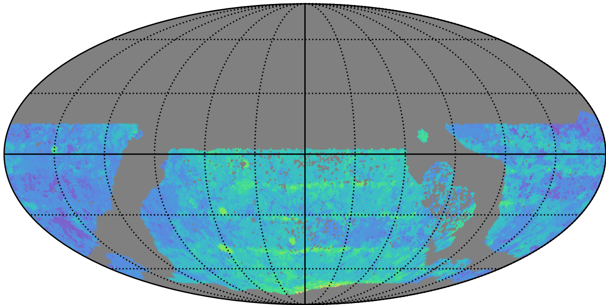
too_ignore_100_4v3.4_10yrs WFD y band: Median Season Length
