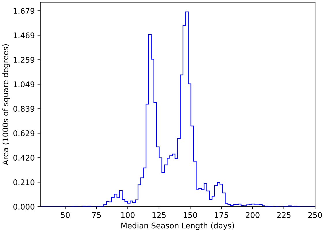
too_ignore_100_4v3.4_10yrs WFD y band: Median Season Length
