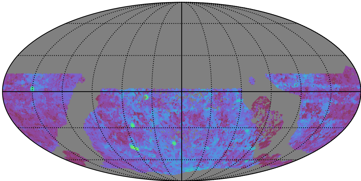
too_ignore_100_4v3.4_10yrs WFD u band: Median Season Length
