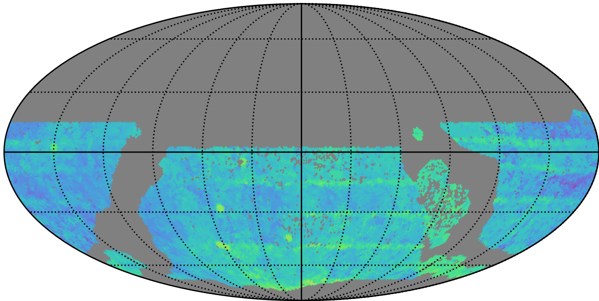
too_ignore_100_4v3.4_10yrs WFD r band: Median Season Length
