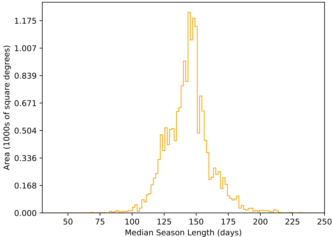
too_ignore_100_4v3.4_10yrs WFD r band: Median Season Length
