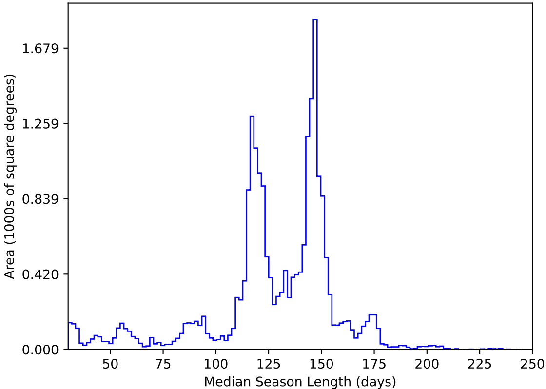
too_ignore_100_4v3.4_10yrs All sky y band: Median Season Length
