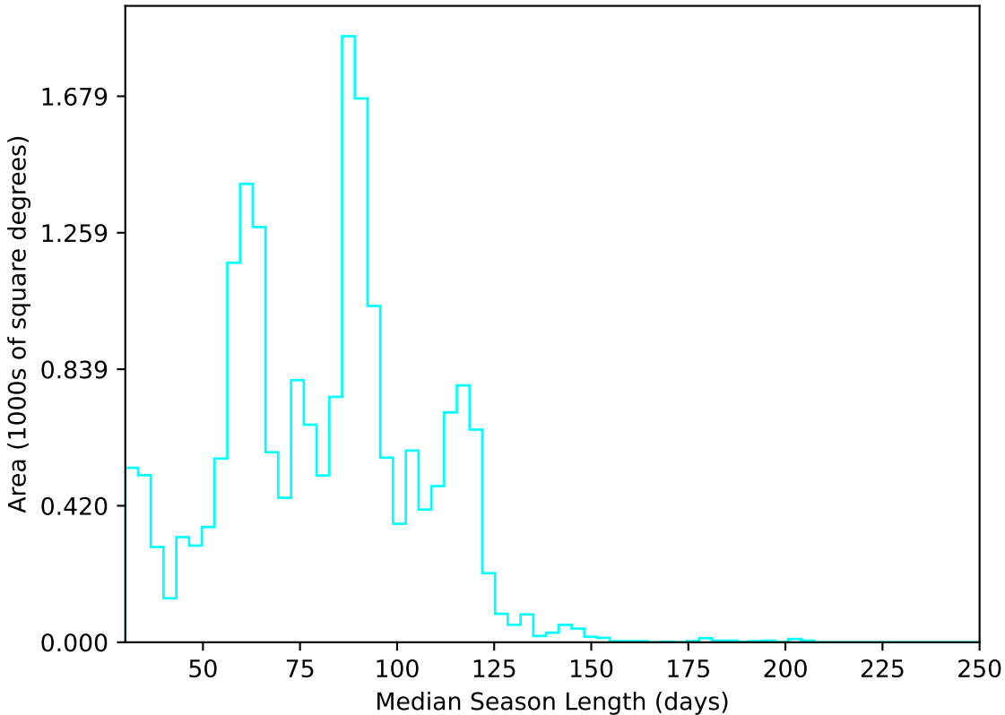
too_ignore_100_4v3.4_10yrs All sky u band: Median Season Length
