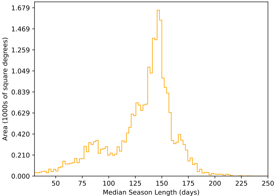
too_ignore_100_4v3.4_10yrs All sky r band: Median Season Length
