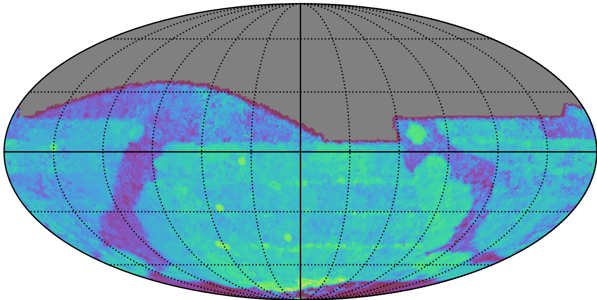
too_ignore_100_4v3.4_10yrs All sky i band: Median Season Length
