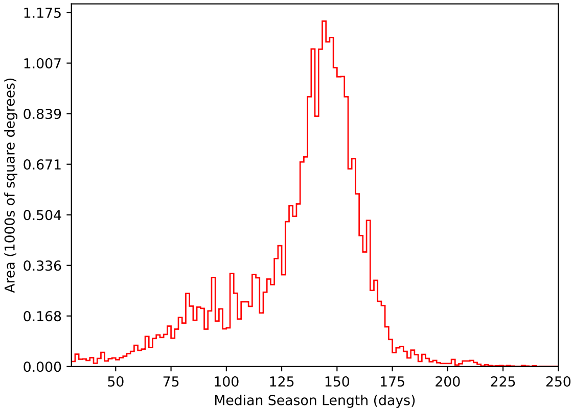
too_ignore_100_4v3.4_10yrs All sky i band: Median Season Length
