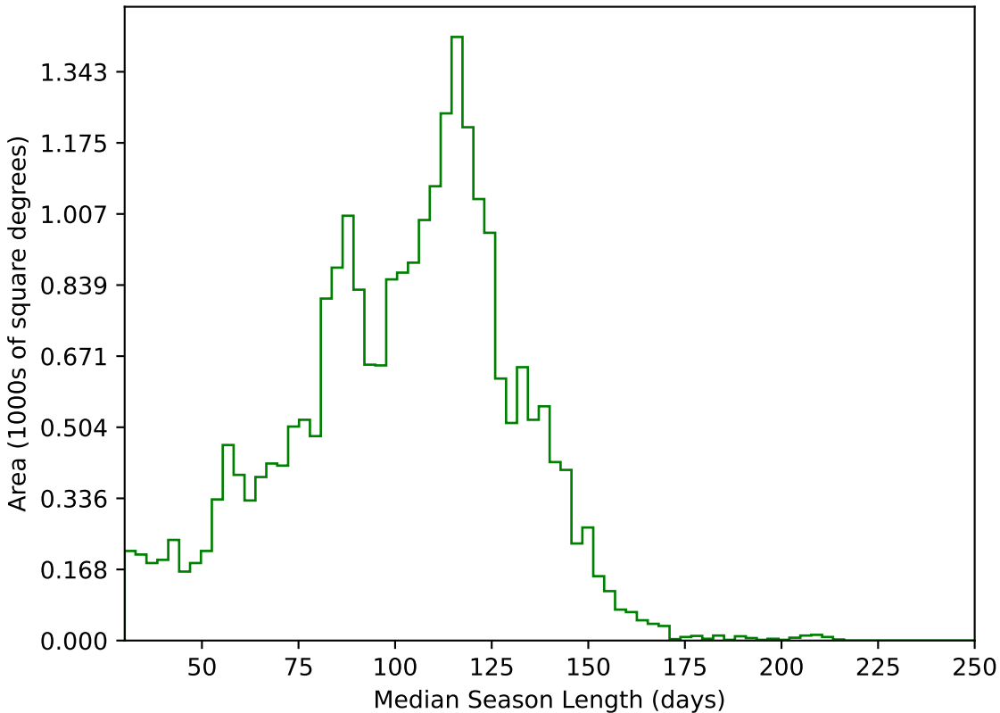
too_ignore_100_4v3.4_10yrs All sky g band: Median Season Length
