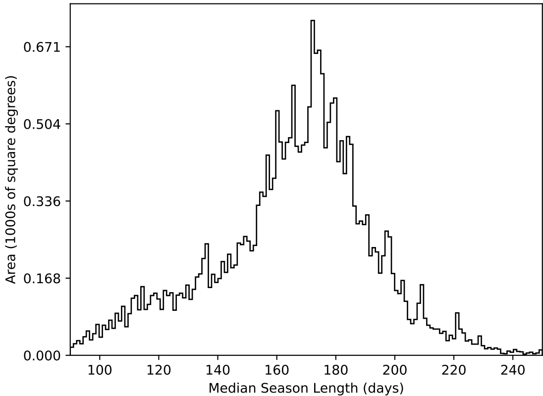
too_ignore_100_4v3.4_10yrs All sky all bands: Median Season Length
