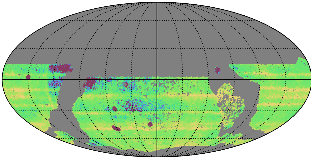
too_ignore_100_4v3.4_10yrs WFD: Median Intra-Night Gap
