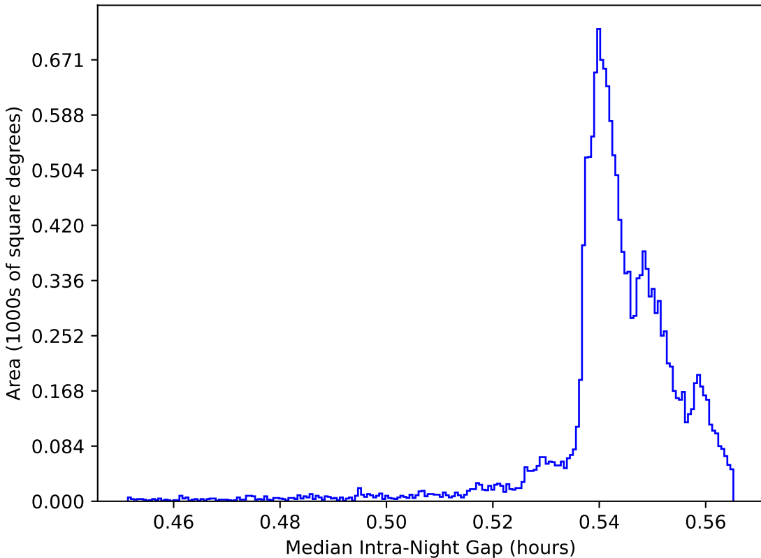
too_ignore_100_4v3.4_10yrs WFD: Median Intra-Night Gap
