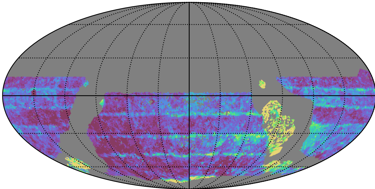
too_ignore_100_4v3.4_10yrs WFD z band: Median Inter-Night Gap
