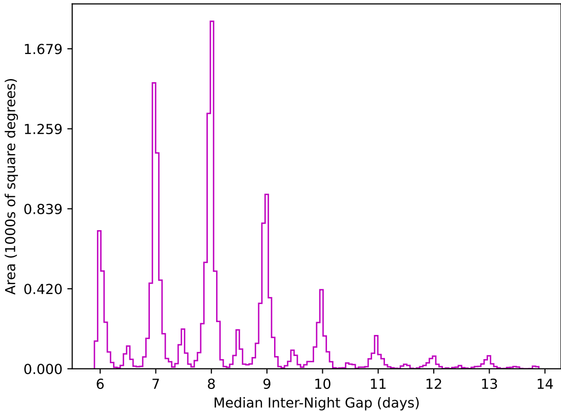
too_ignore_100_4v3.4_10yrs WFD z band: Median Inter-Night Gap
