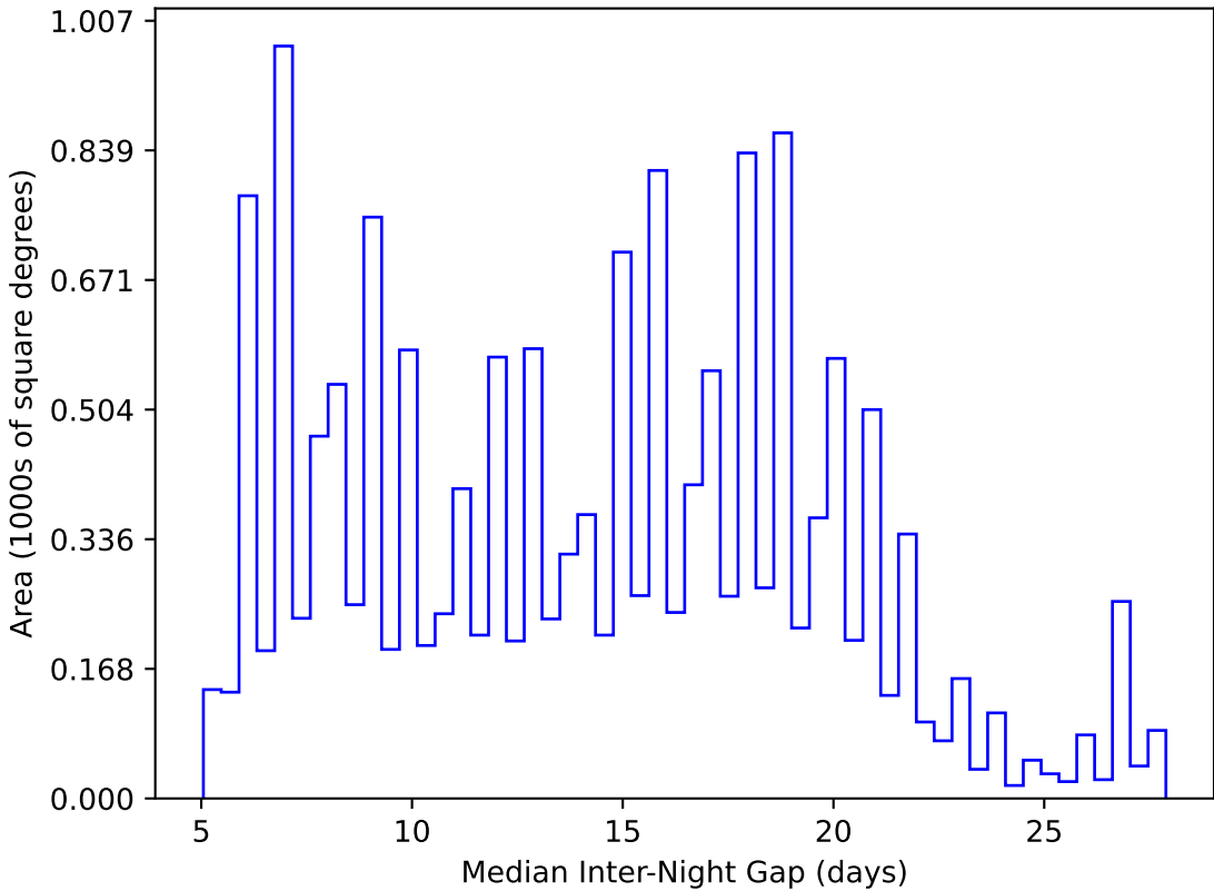
too_ignore_100_4v3.4_10yrs WFD y band: Median Inter-Night Gap
