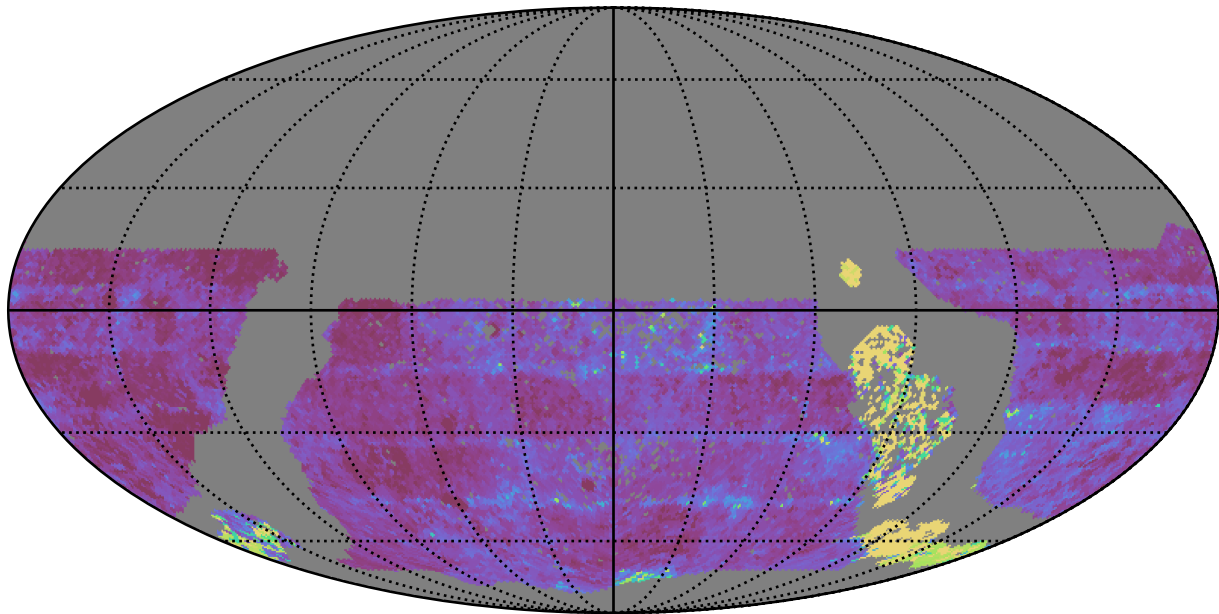
too_ignore_100_4v3.4_10yrs WFD u band: Median Inter-Night Gap
