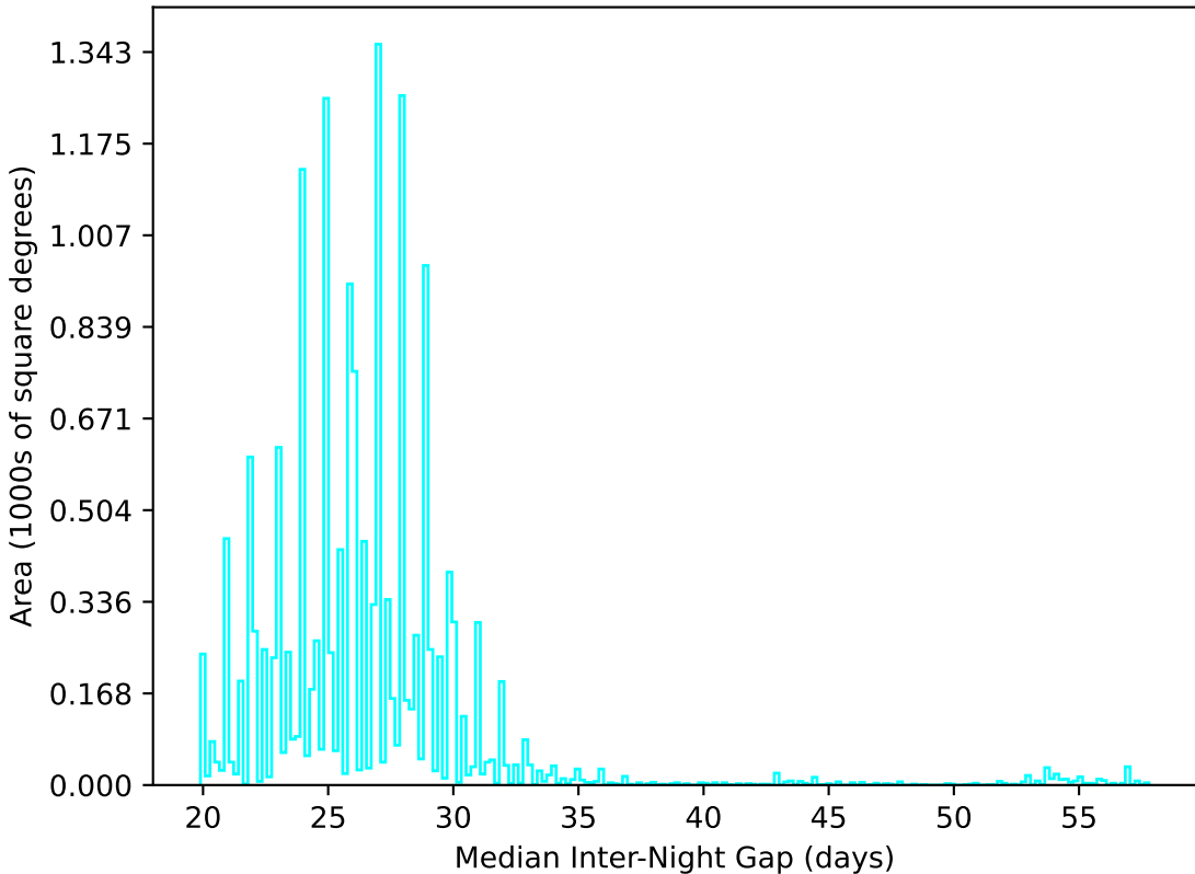
too_ignore_100_4v3.4_10yrs WFD u band: Median Inter-Night Gap
