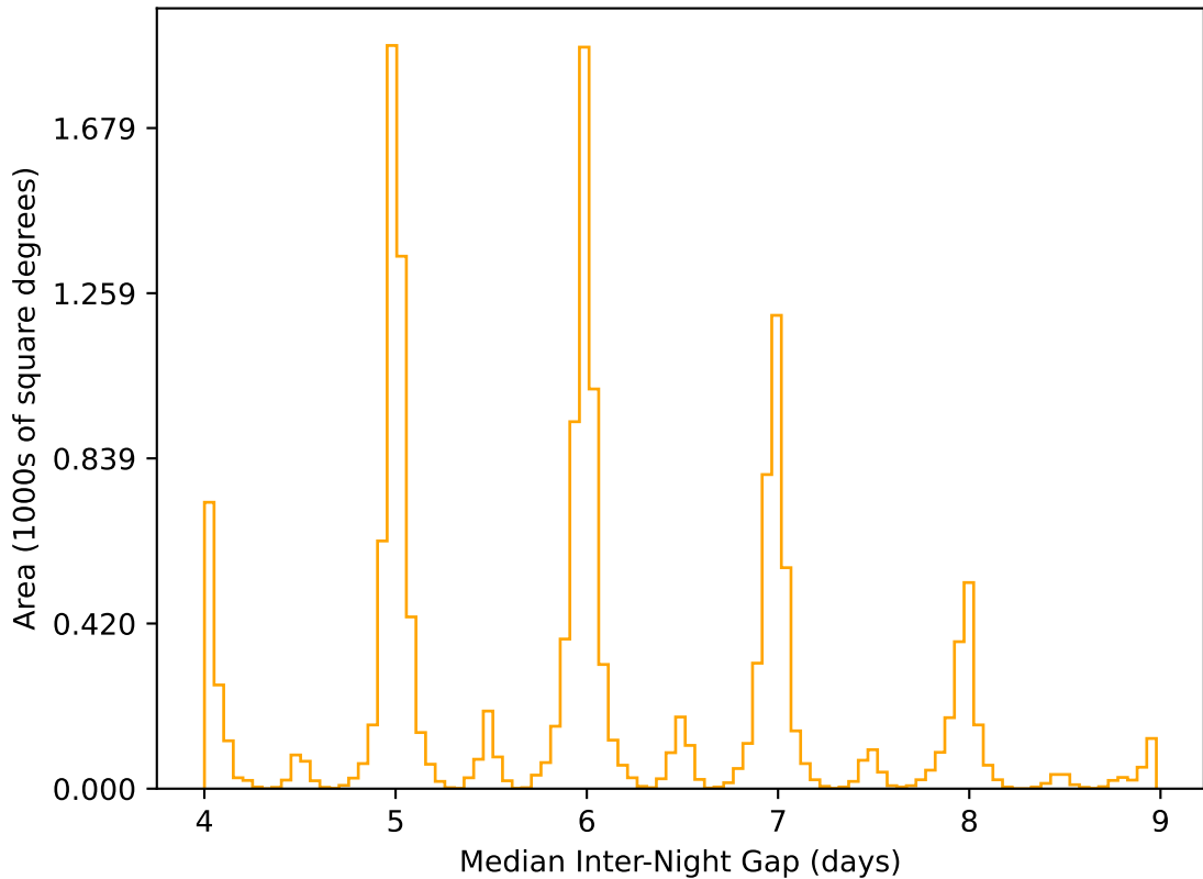
too_ignore_100_4v3.4_10yrs WFD r band: Median Inter-Night Gap
