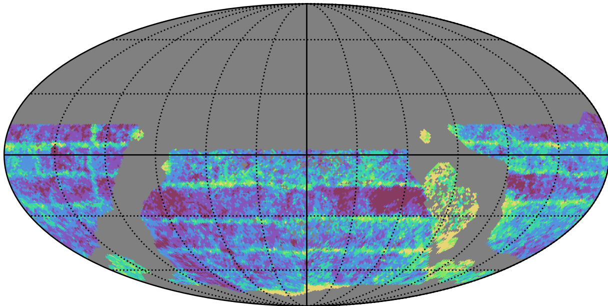
too_ignore_100_4v3.4_10yrs WFD i band: Median Inter-Night Gap
