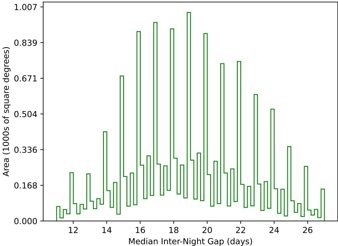
too_ignore_100_4v3.4_10yrs WFD g band: Median Inter-Night Gap
