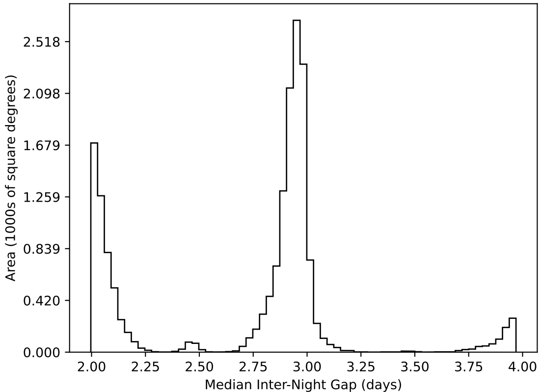
too_ignore_100_4v3.4_10yrs WFD all bands: Median Inter-Night Gap
