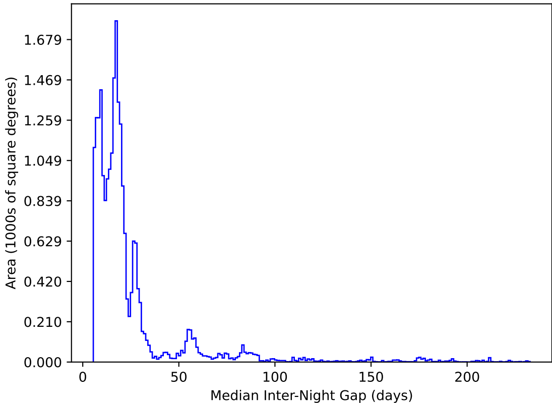
too_ignore_100_4v3.4_10yrs All sky y band: Median Inter-Night Gap
