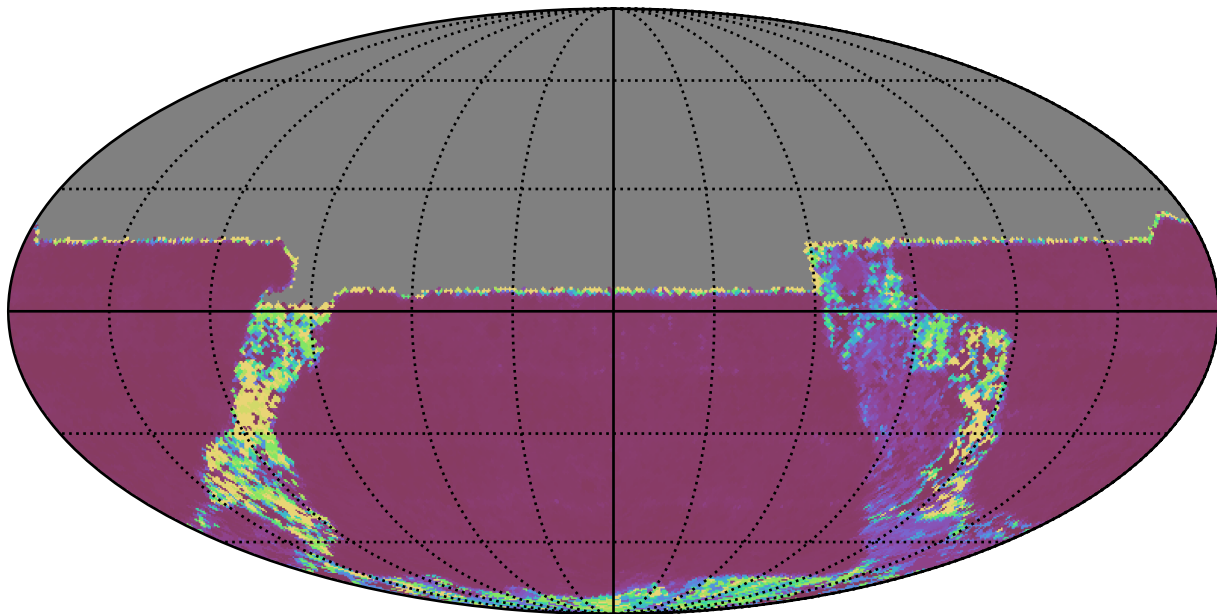
too_ignore_100_4v3.4_10yrs All sky u band: Median Inter-Night Gap
