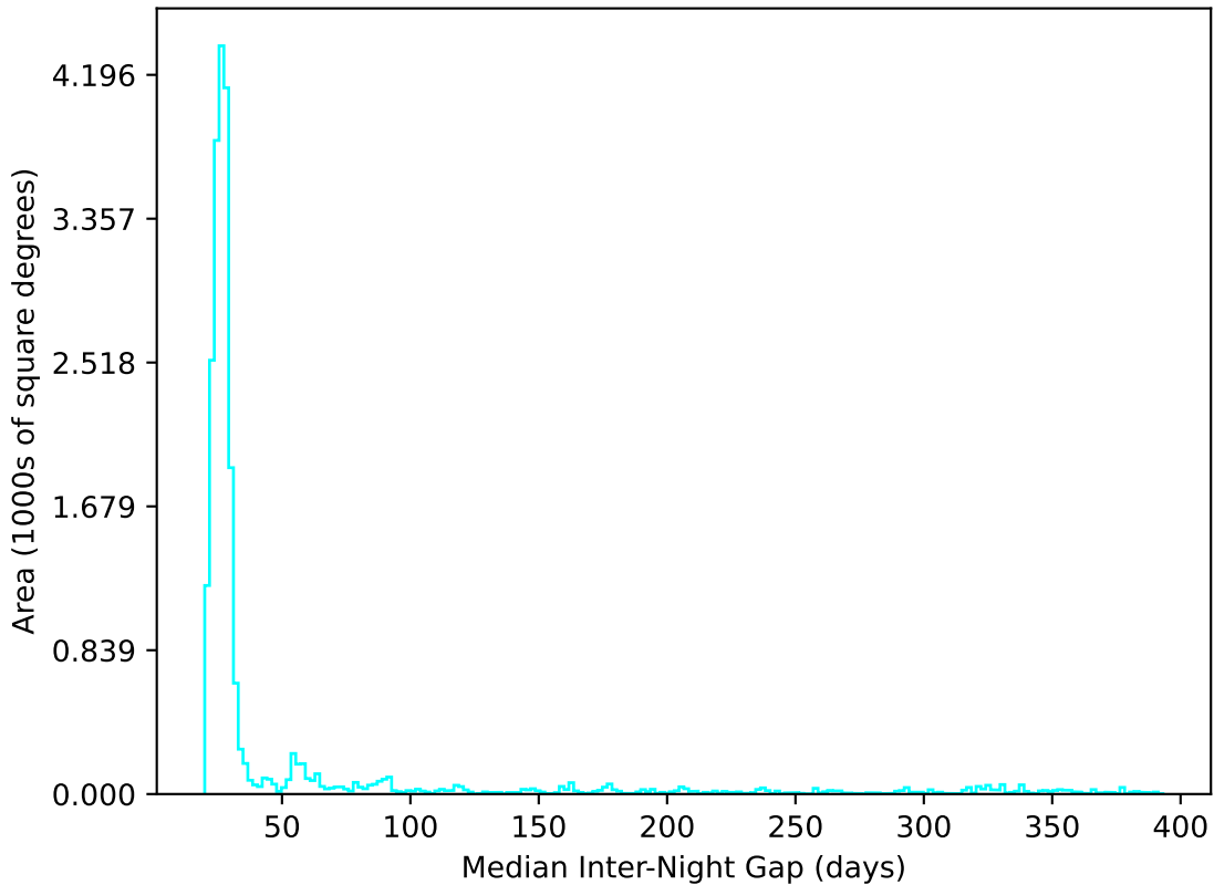
too_ignore_100_4v3.4_10yrs All sky u band: Median Inter-Night Gap
