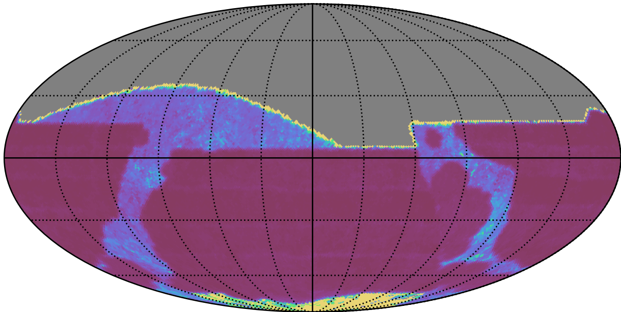
too_ignore_100_4v3.4_10yrs All sky r band: Median Inter-Night Gap
