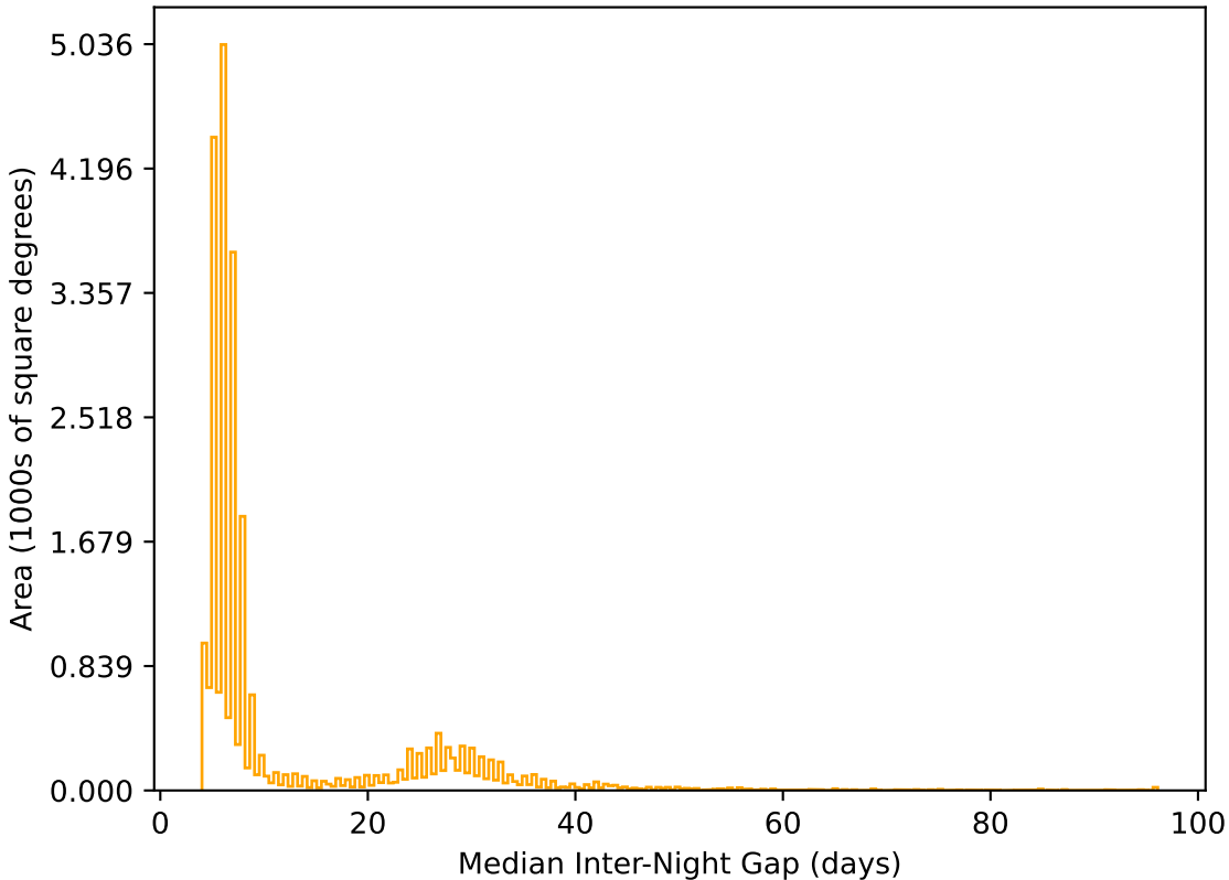
too_ignore_100_4v3.4_10yrs All sky r band: Median Inter-Night Gap
