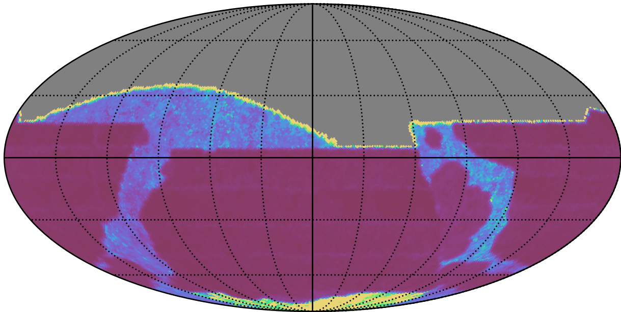
too_ignore_100_4v3.4_10yrs All sky i band: Median Inter-Night Gap
