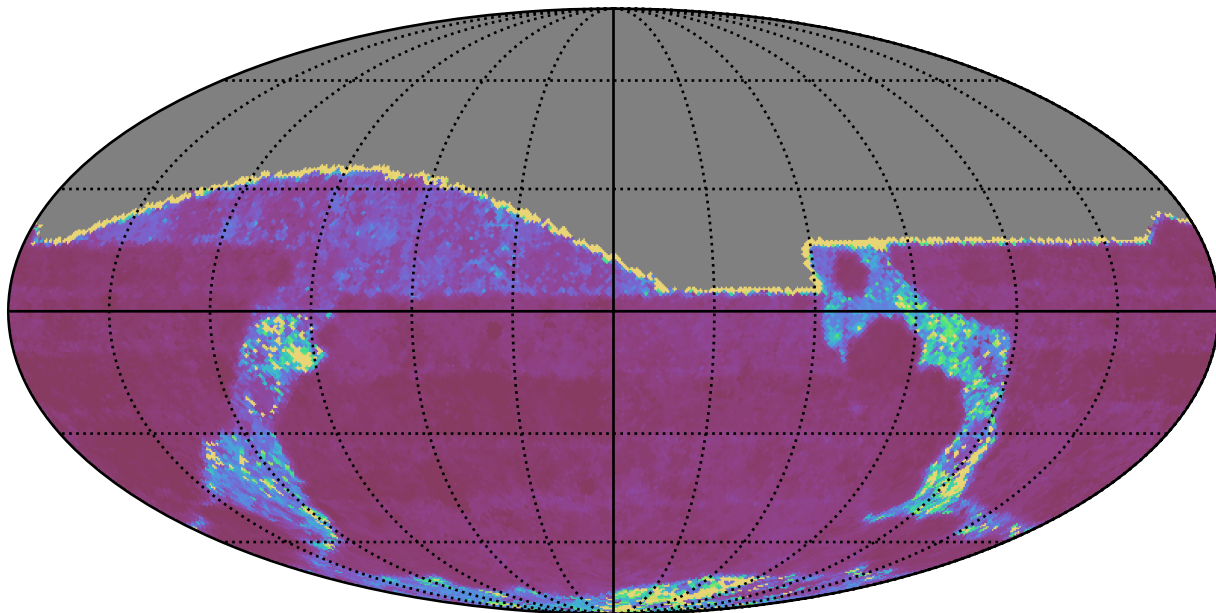
too_ignore_100_4v3.4_10yrs All sky g band: Median Inter-Night Gap
