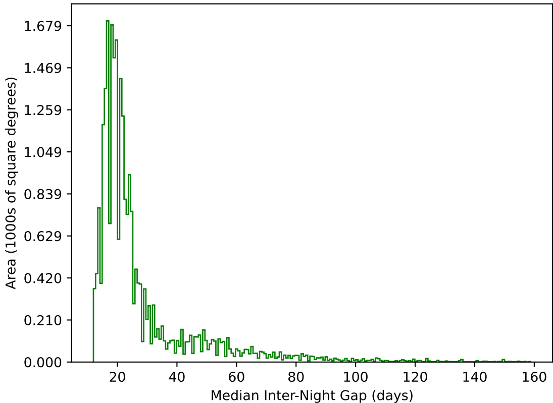
too_ignore_100_4v3.4_10yrs All sky g band: Median Inter-Night Gap
