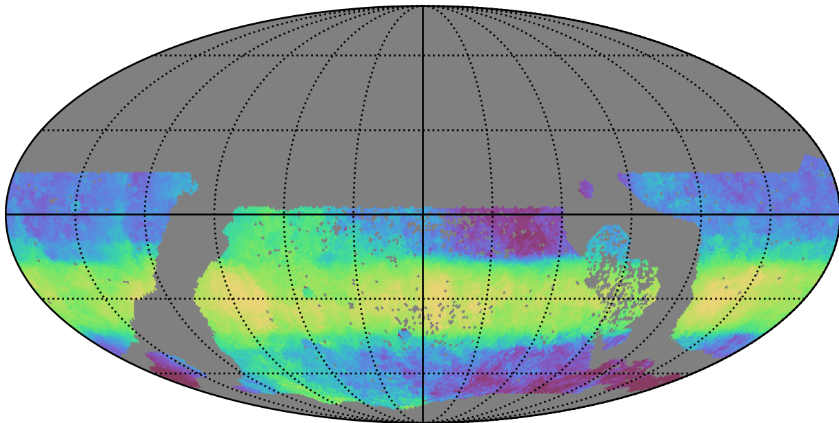
too_ignore_100_4v3.4_10yrs WFD z band: Median HA
