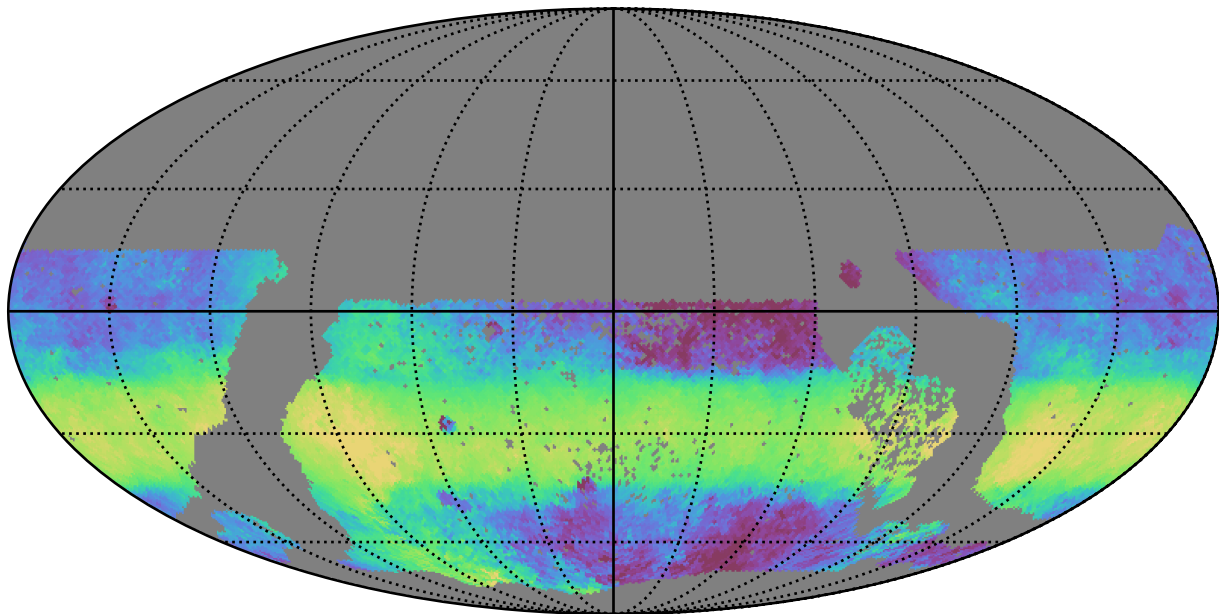
too_ignore_100_4v3.4_10yrs WFD y band: Median HA
