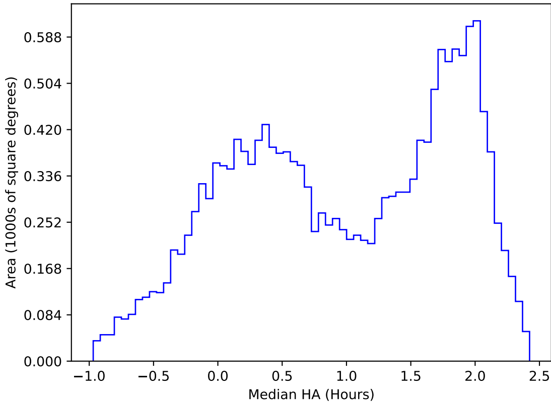
too_ignore_100_4v3.4_10yrs WFD u band: Median HA
